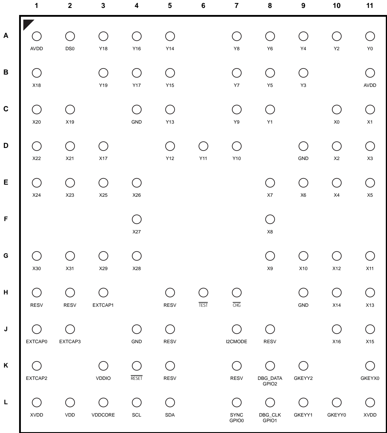
Top View
